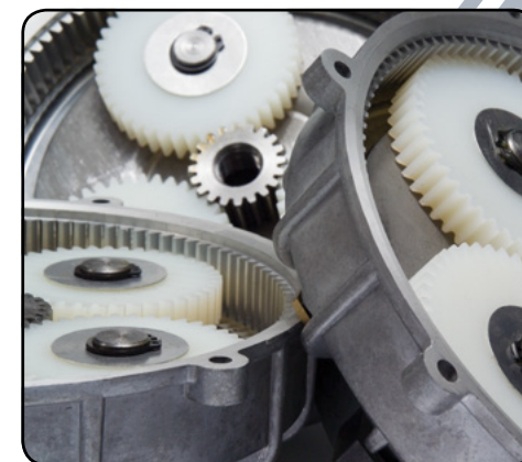
Planetary gearbox
